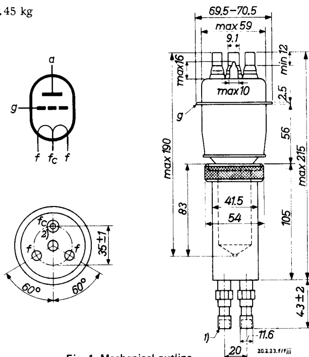
Fig. 1 Mechanical outline.
